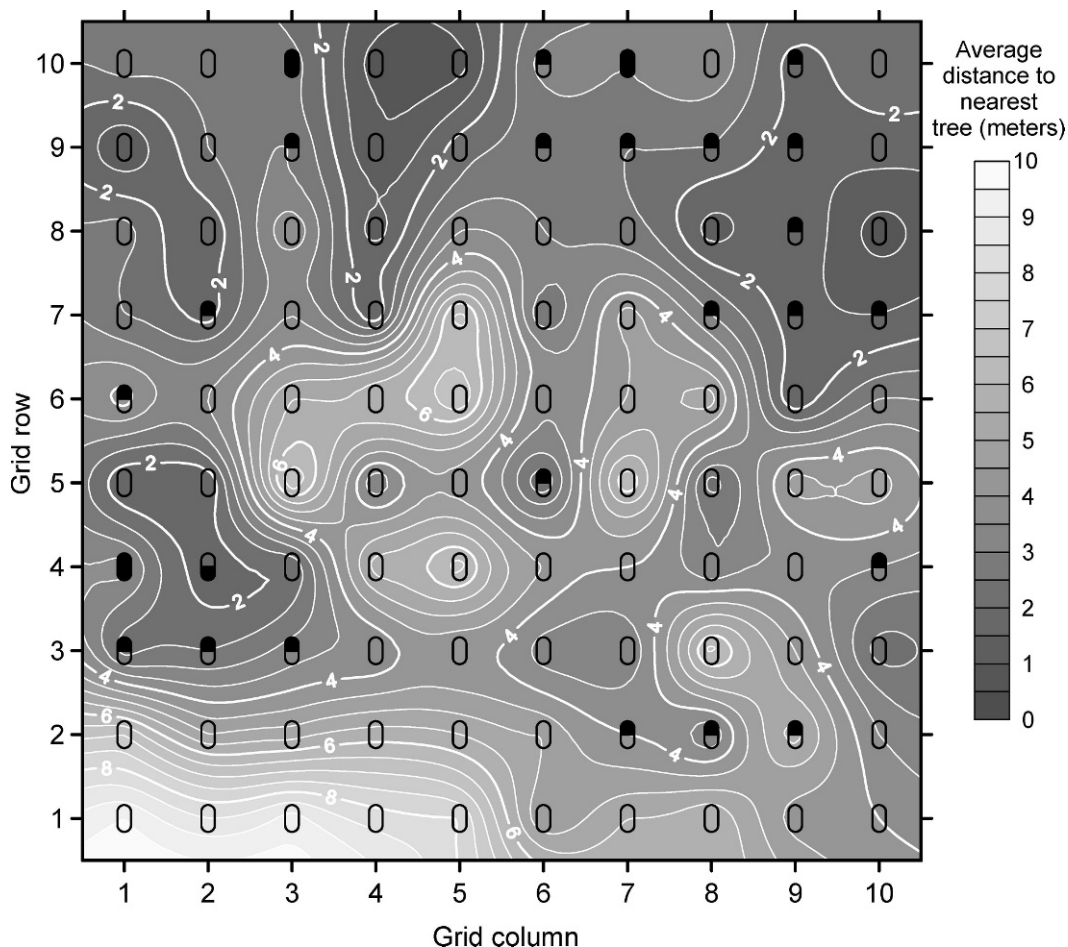
FIG. 2—Depiction of grid 2 in 2004 showing stations where tawny deer mouse ( Peromyscus perfulvus ) was caught and not caught. Solid black ovals indicate where tawny deer mouse was captured in both arboreal and ground traps. If only top half of oval is filled, tawny deer mouse was caught only in arboreal trap; if only bottom of oval is filled, tawny deer mouse was caught only in ground trap. Unfilled oval indicates species was not caught at station. Contours signify estimated average distance to nearest tree, with surface determined through use of kriging based on measurements taken at the 100 trap stations.
